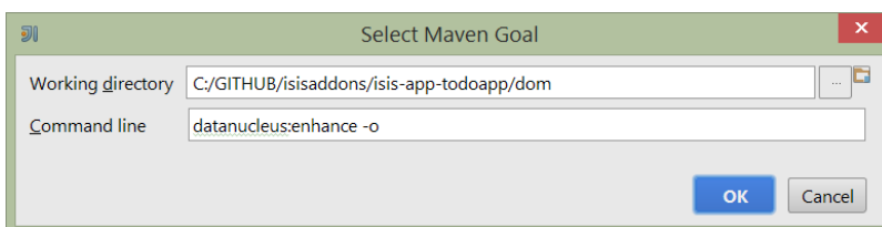
Figure 28. IntelliJ Running the App - Datanucleus Enhancer Goal
